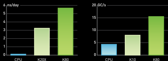
Life Science: AMBER 2 Benchmark
